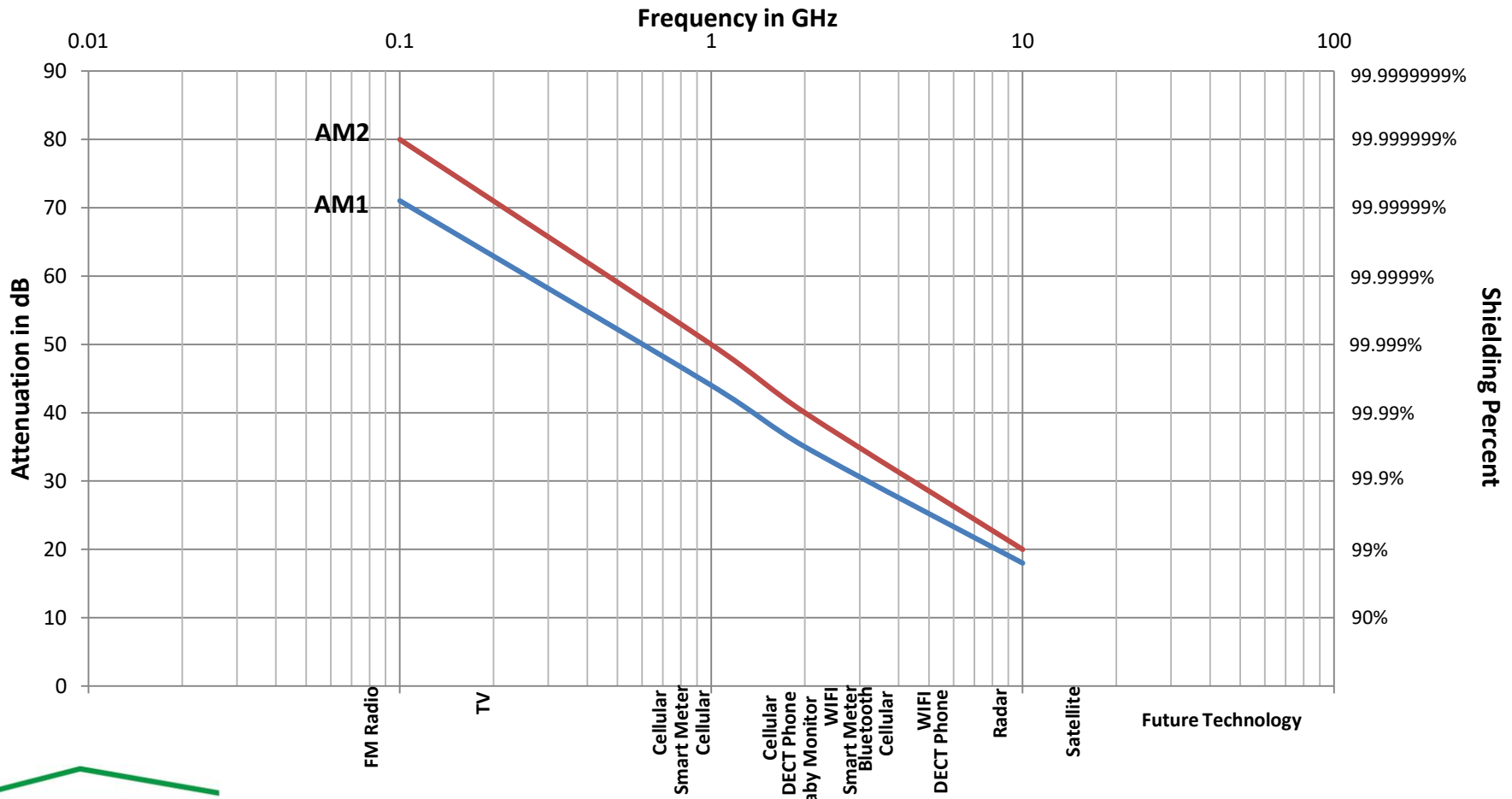
Wire Mesh RF Shielding Performance - 1 Layer
